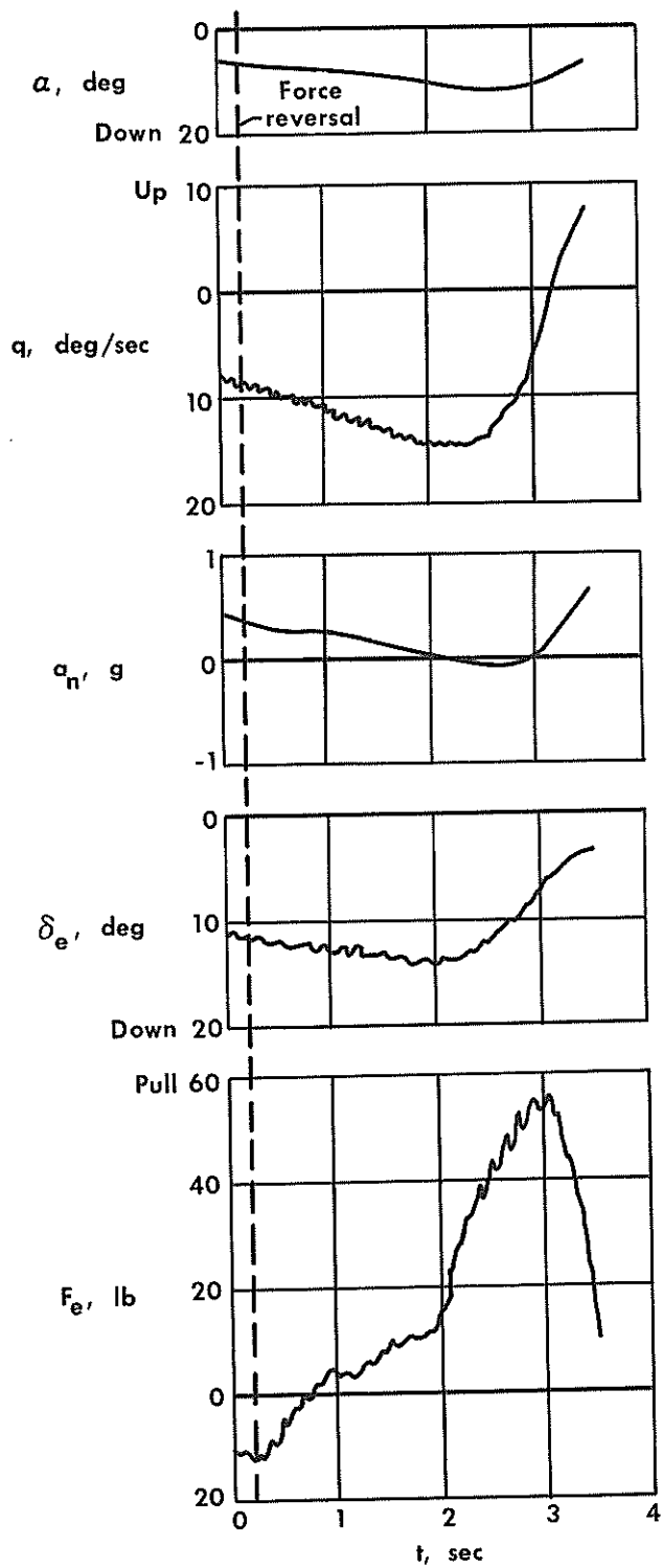
Figure 12.— Time history of pertinent longitudinal parameters during force reversal shown in figure 11. Landing configuration; aft center of gravity; V_C = 72 knots.
