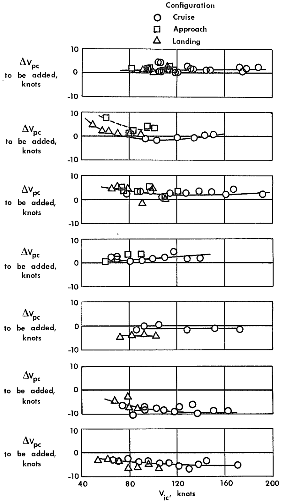
Figure 3.— Airspeed position-error calibration for all airplanes tested.
