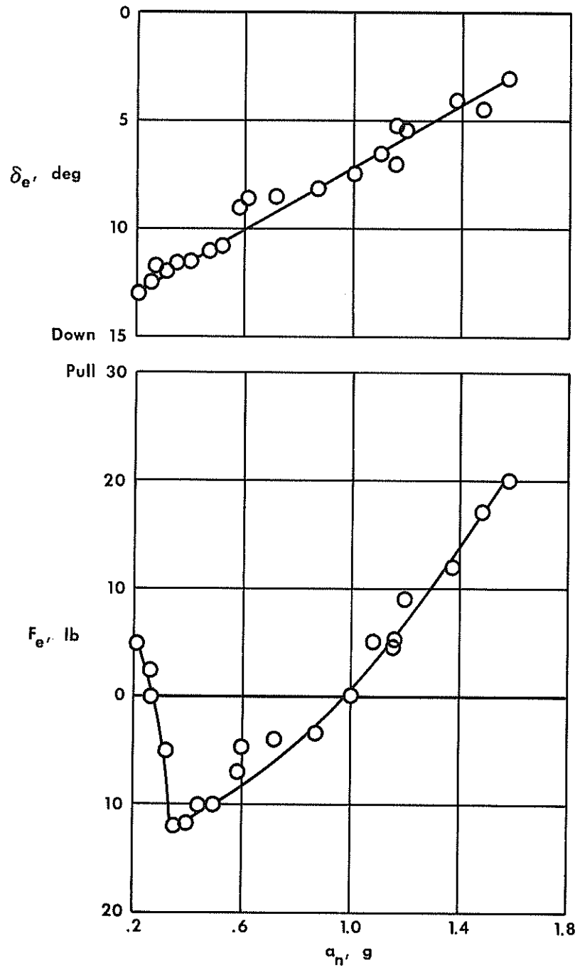
Figure 11.— Example of elevator force reversal, landing configuration; aft center of gravity; V_0 = 72 knots.
