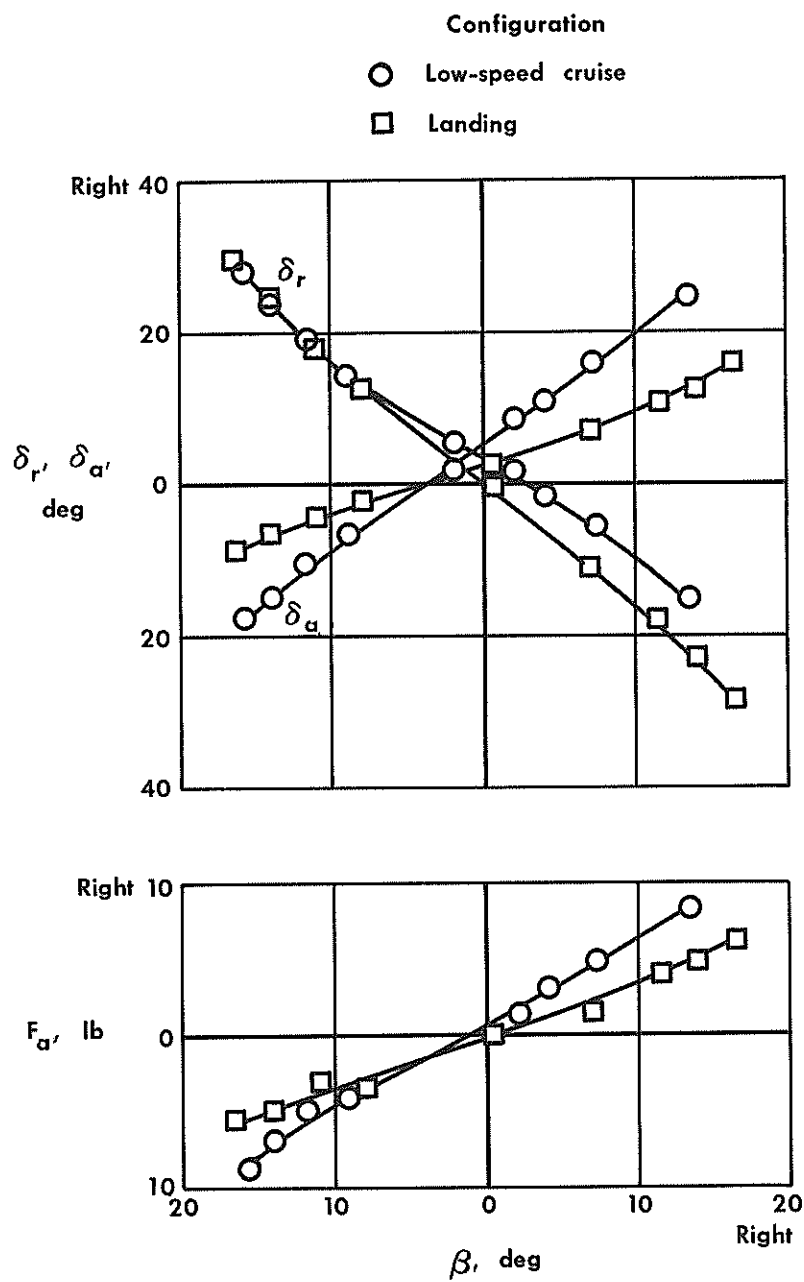
(a) Effect of configuration. V_c = 89 knots.
