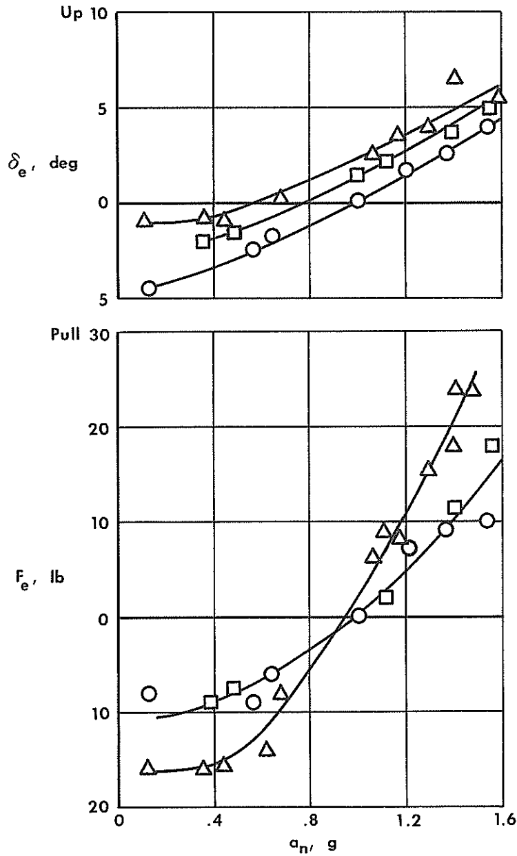
(b) Maneuvering stability. V_e = 97 knots.
